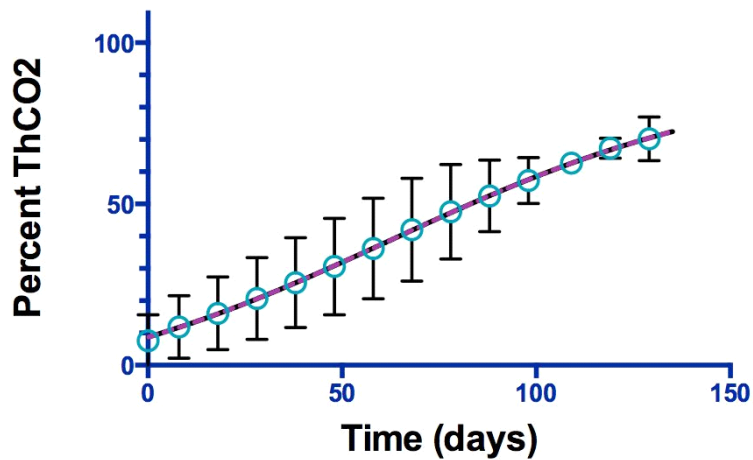
Figure - Test chamber carbon dioxide (CO 2 ) measurement as the percent of theoretical maximum (% ThCO 2 ) derived from the test sample. Average values are plotted with the standard deviation (+/- SD) for the time course of the test. Curve fit is applied to calculate the statistical confidence for 95% (line) and predicted (red) curve fit.
